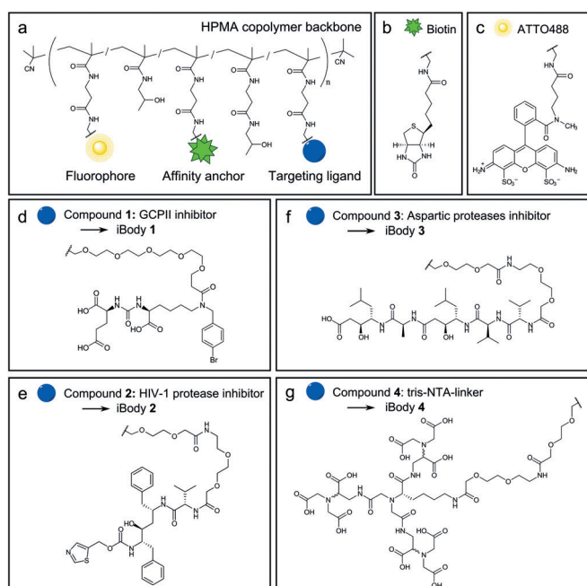
Figure 1. Structures of the iBodies and their functional modules. a) HPMA copolymer decorated with functional modules. b) The affinity anchor biotin. c) ATTO488 fluorophore. d) GCPII inhibitor. e) HIV-1 protease inhibitor. f) A class-specific inhibitor of aspartic proteases. g) A nitrilotriacetic acid (NTA)-based ligand for binding the His-tag.
